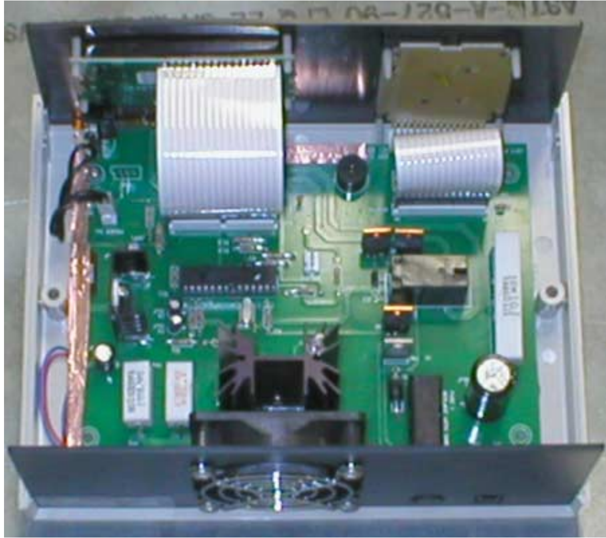
Figure 3: View of Controller PCB mounted in enclosure
